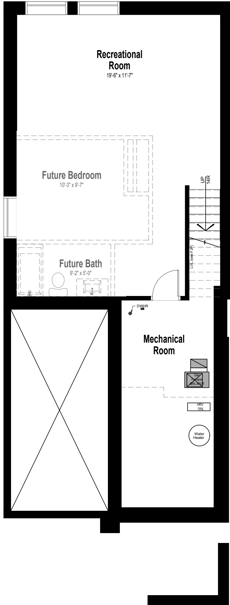
1 BASEMENT PLAN
